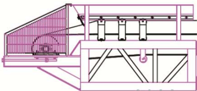
TENSIONING UNIT
