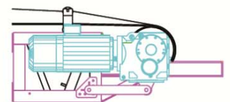
DRIVING UNIT
